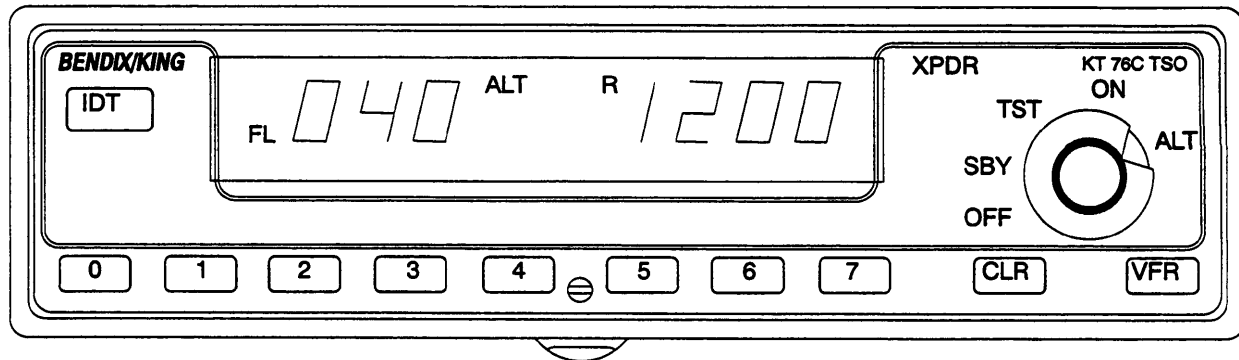
FIGURE 3-8 Altitude Display
