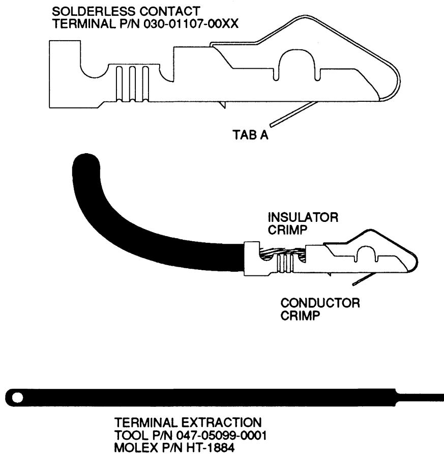
FIGURE 2-1 Crimping Tool (Sheet 1 of 3)
