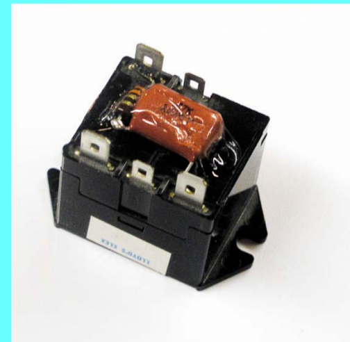
----Generator/Dynamo/Alternator Control Relay----
