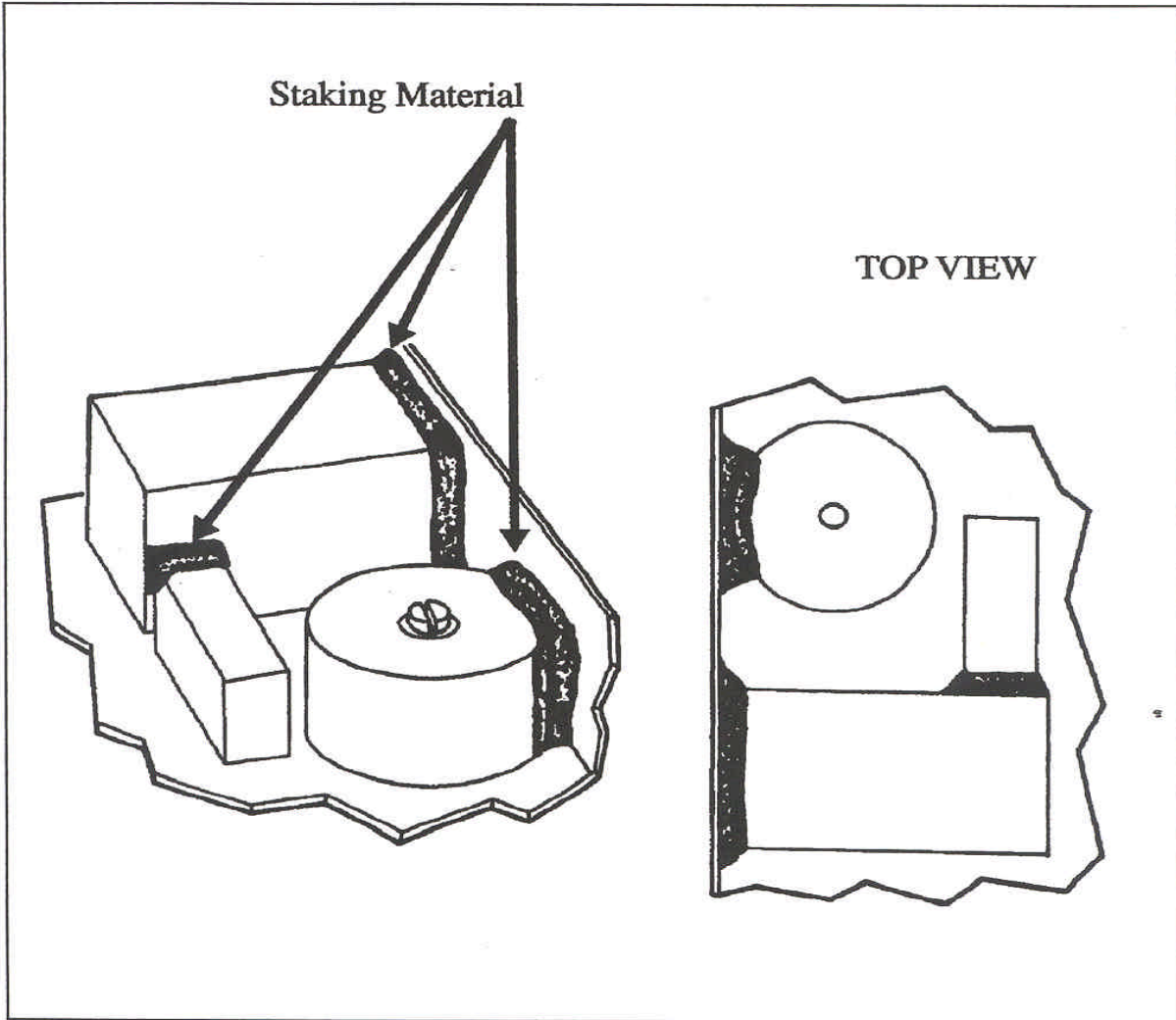
Figure 9-10: Vibration Isolation Staking
