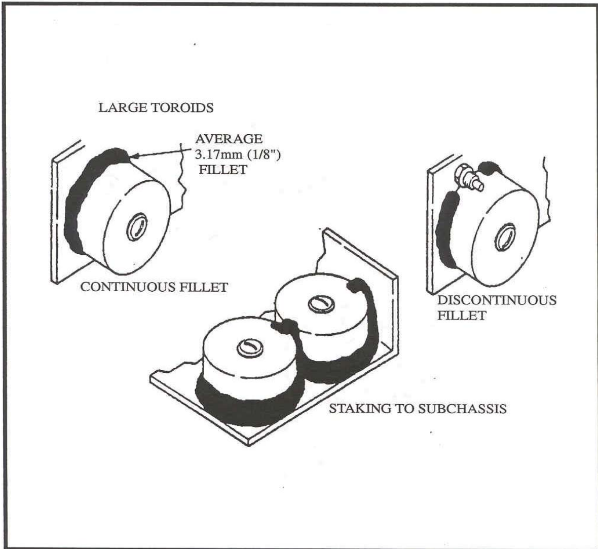
Figure 9-9: Toroid Staking
