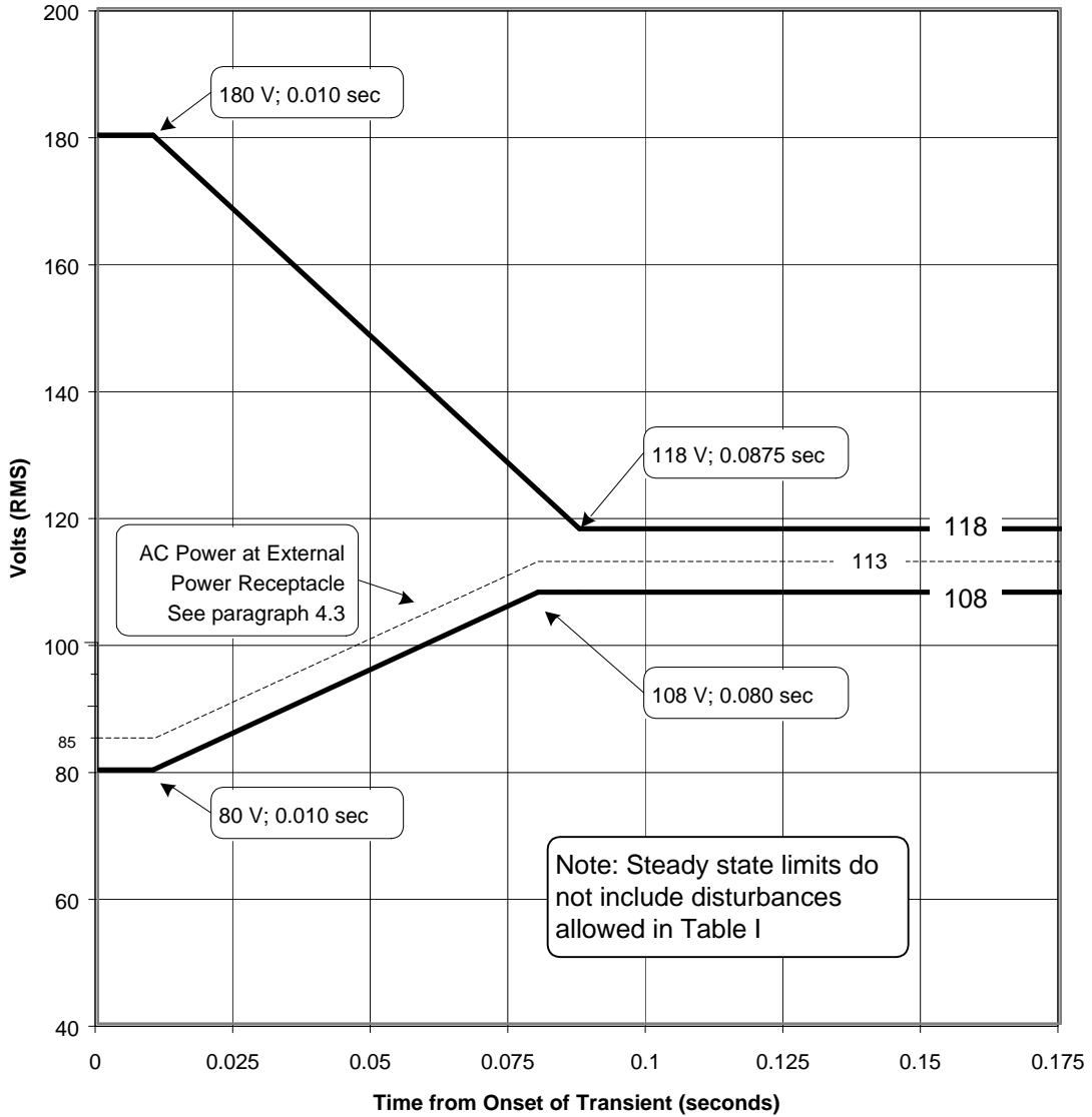
FIGURE 3. Envelope of normal 400 Hz and variable frequency AC voltage transient.
