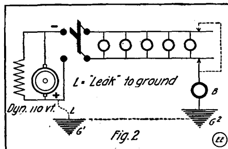
Fig. 2. Causes of Low Voltage Shocks Due to Accidental "Grounds" at Two Points on the Line.
