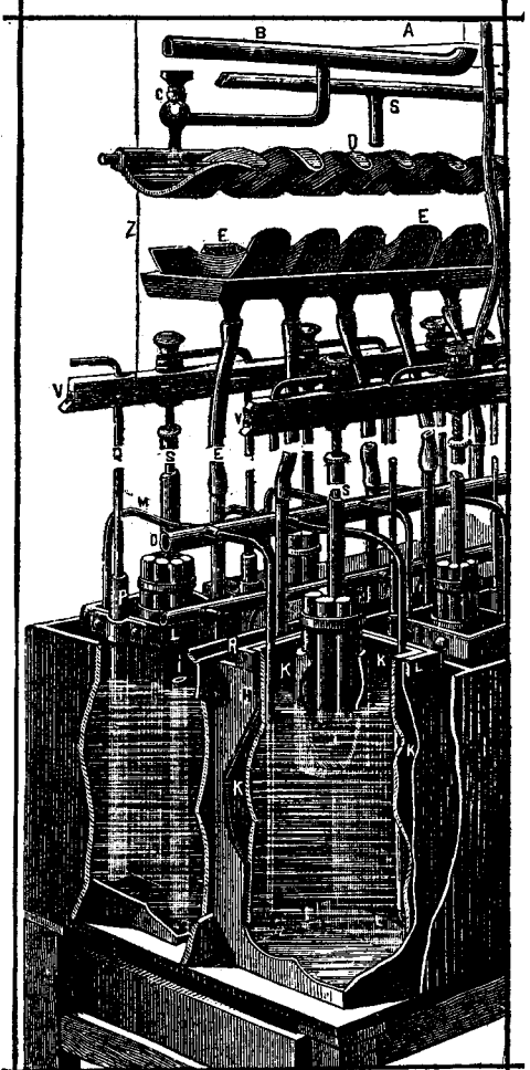
Fig. 2. Detailed View of Early Power Battery. It Was of the Primary Type and Was Charged with Chemicals.
