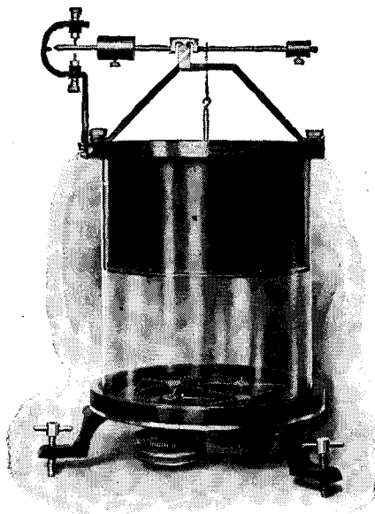
This Motor Driven Mechanical Device Illustrates in a Vivid Manner the Molecular Action in Gases
