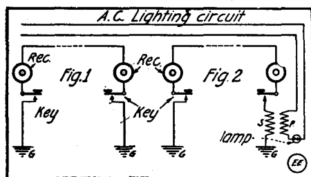
The Current for Operating This Telephone and Telegraph System Is Obtained Inductively from the A.C. Lighting Circuit.
