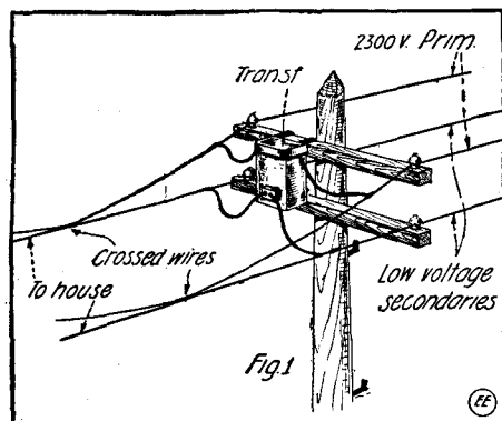
Fig. 1. Showing How High Voltage Wires May Drop onto Low Voltage House Service Lines, Thus Charging the Latter to a Dangerous Potential. This Cause Was Responsible for the Death of Mr. C. F. Purick of Port Jefferson, L. I.
