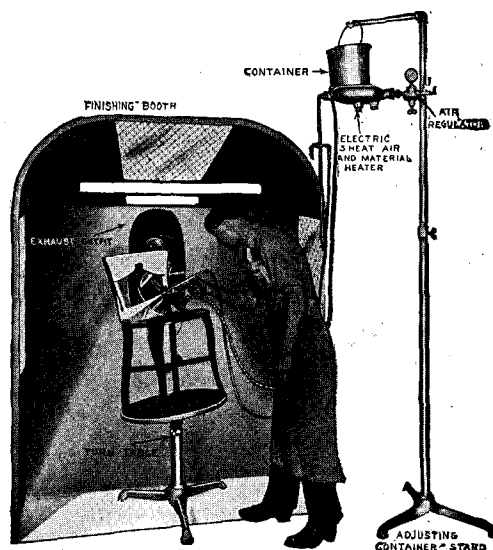
Electric Air Brush Outfit for Finishing Chairs.
