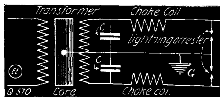
Static Interrupter Protector for High Tension Transformer Lines
