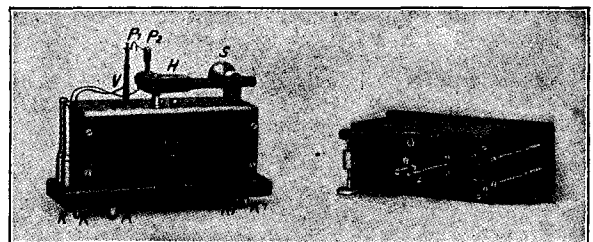
Fig. 2. Vibrating "Tikker" for Undamped Wave Reception. Employs Two Gold Wires for Interrupting 'Phone Circuit.
