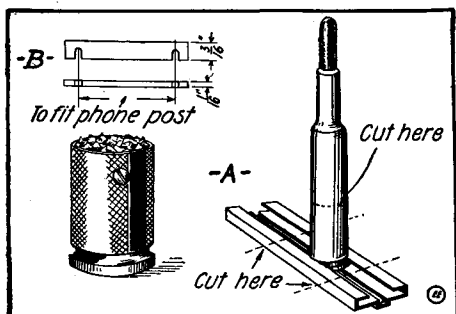
Revolvable and Removable Detector Cup Made from Cartridge Shell.
