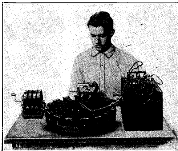
Clever Battery Magnetizer Recharging a Ford Magneto.
