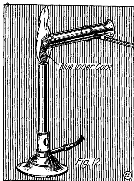
In Heating a Test Tube Containing Solution Place It in Blue Flame of Bunsen Burner.
