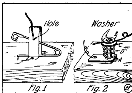
Simple Yet Effective Wire Connectors of Home-Made Construction.
