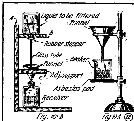
Two Schemes for Filtering Liquids.
