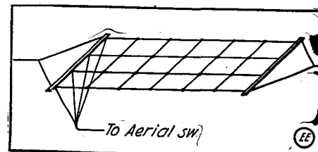
An Efficient Aerial Design.
