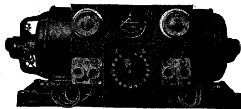
Battery-Charging Motor-Generator with Steel Switch Panel.
