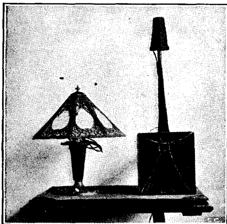
Photo by courtesy of the International Callophone Corporation. The Lamp at the Left Contains a Microphone and Loud-Talker; Improved Loud Talker with Horn at Right.
