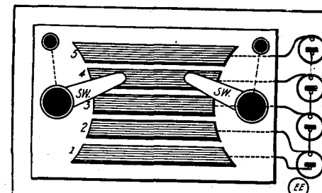
Handy Pole-Changing Switch Made of Two Switch Blades and Metal Strips
