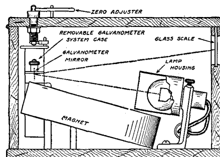
Interior View of Compact Mirror Galvanometer.
