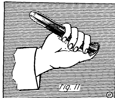
Shaking Liquids in a Test Tube, Closing the Opening with the Thumb.
