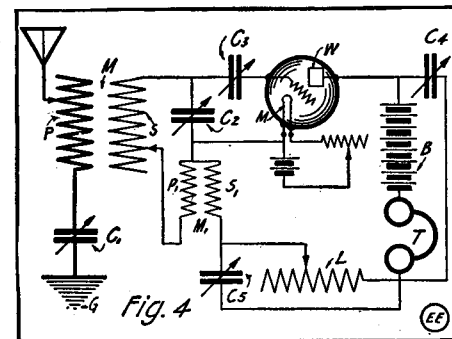
A Second Method of Arranging an Audion Detector to Interpret Continuous Wave Signals.
