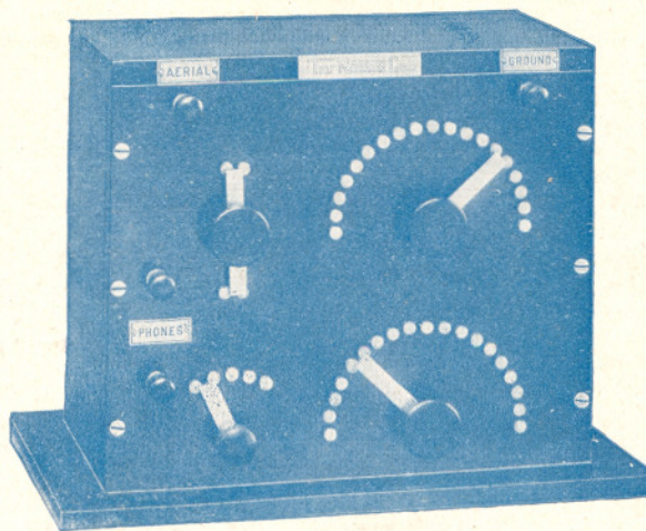
COMPLETE EVER-READY RECEIVING STATION Type A
