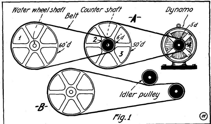
Diagram Showing Relations Between Various Pulley Diameters and Speeds, Also How an "Idler" Pulley Can Be Used Advantageously in Short Drives to Increase Belt Contact.
