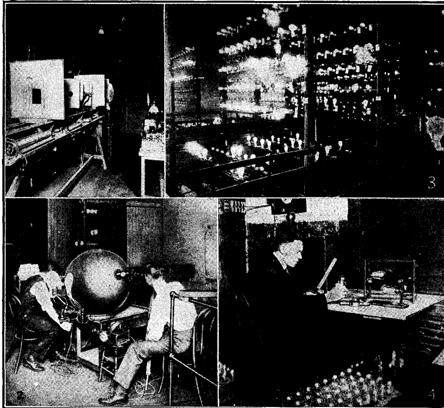
Fig. 1. Shows a Photometer for Measuring the Candle-power of Incandescent Lamps. Fig. 2 a Spherical Photometer for Similar Work. Fig. 3. "Life" Test Racks. Fig. 4. Lamp Inspector at Work.
