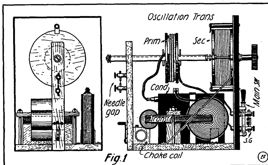
Efficient Design for 100-Watt A. C. Transformer Panel Type Control Radio Sending Set. Note Compactness, with Consequent Short Lead Connections. Oscillation Transformer May be Adjusted by Knob on Front of Panel. A Hot-wire Ammeter may be Mounted at the Top of the Panel to Indicate the Radiation Current.
