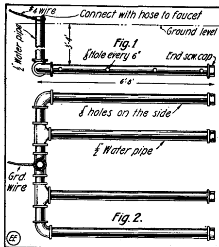
By Pouring Water Down Thru This Multiple Pipe "Ground" a Good Earth Connection Is Assured.
