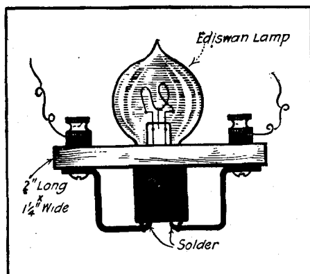
Efficient Manner of Using Edison Screwless Base Battery Lamps by Soldering Two Wires to the Base Terminals.
