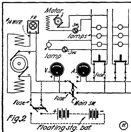
Typical Isolated Electric Lighting Plant, with Measuring Instruments, Voltage Regulator and Distribution Circuit Switches.
