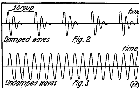
How Damped Waves Differ From Undamped Waves as Used in Radio-Telegraphic Transmission station a note or tone corresponding to the middle C on the piano.
