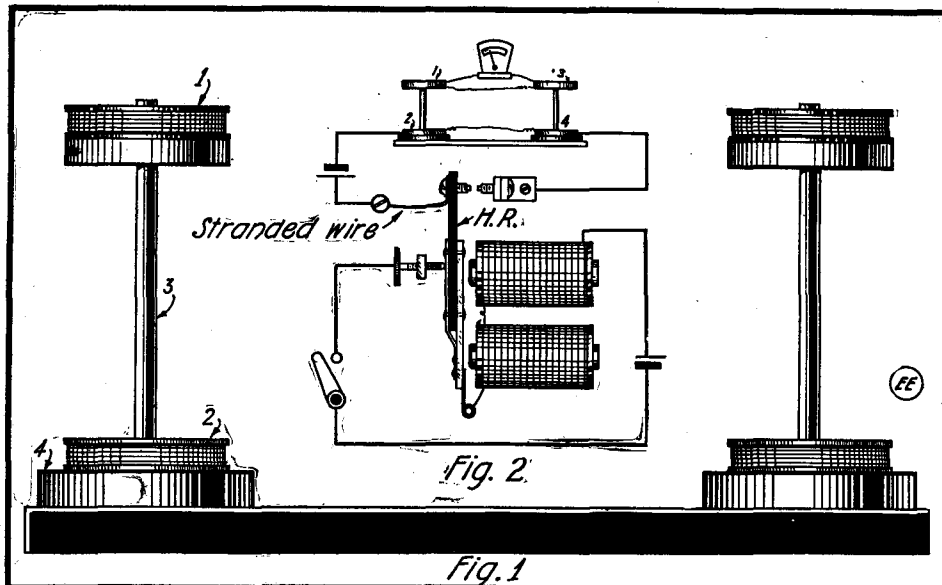
Fig. 1 An Induction Balance Whereby Difference in Coins, Such as "Counterfeit" Can Be Quickly Detected. Normally the Two Upper Coils "Buck" the Two Lower Ones, Giving Zero Deflection on the Galvanometer.
