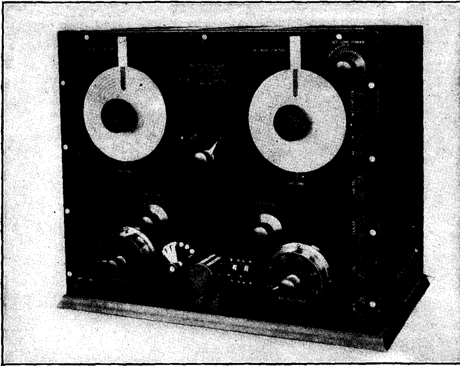
Latest De Forest Radio Receiving Set With Calibrated Inductance and Condenser Knobs Enabling The Wave Length of an Incoming Signal to Be Instantly Determined. Adapted to Damped and Undamped Waves.
