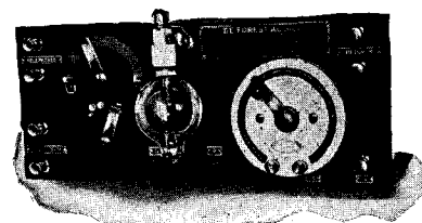
THE TYPE RJ9 DE FOREST AUDION DETECTOR
