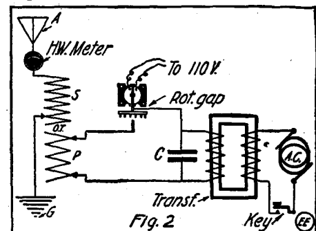
Proper Connections for A. C. Transformer Radio Sender, with Rotary Gap and Oscillation Transformer.
