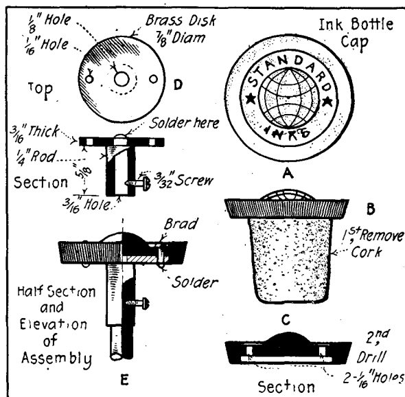
Constructing a Serviceable Switch Knob from Ink Bottle Cork.
