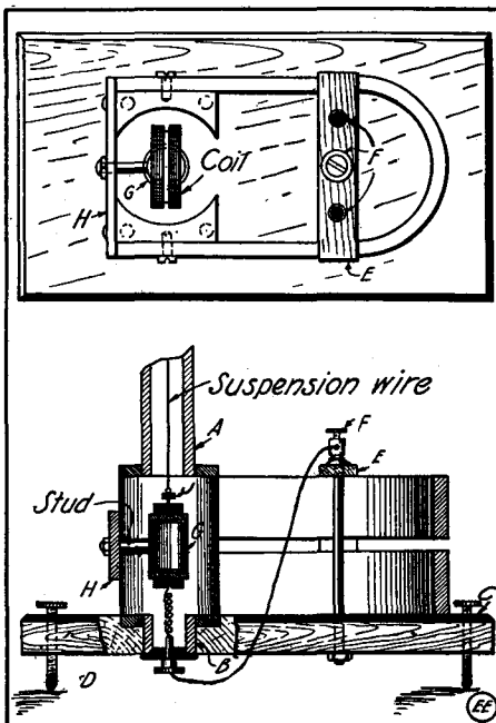
Fig. 3 How a Two Bar Magneto was Converted Into a Sensitive Galvanometer. An Instrument Every Experimenter Should Have.
