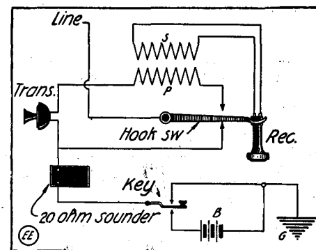
Simple Hook-Up for Telephoning Over Telegraph Lines
