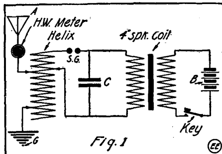
Hook-Up for Spark Coil Radio Transmitter Excited by Battery
