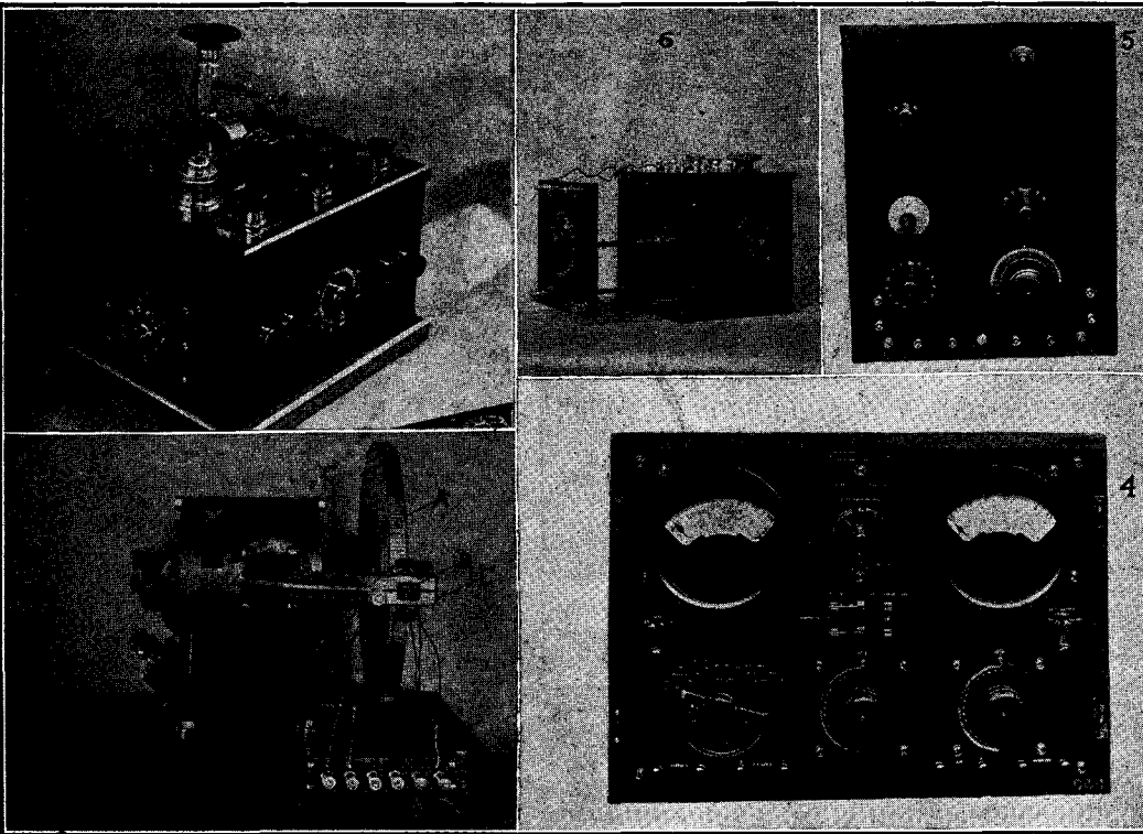
Fig. 1. New Crystal Detector; Fig. 3. Radio Frequency Alternator for "Beat" Receiver; Fig. 4. Calibrated Control Panel for Arc Used with Heterodyne; Fig. 5. Oscillating Audion Panel for Undamped Wave Reception and Fig. 6. Improved Loose Coupler with Pancake Windings.
