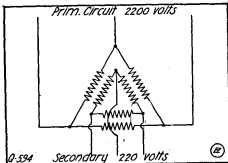
Delta Connection of Three Transformers on a Three Phase A. C. System.
