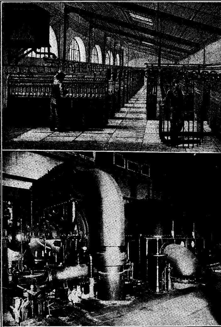
Fig. 1. First We See (Above) One of the Greatest Electric Novelties of a Half-Century Ago, a Huge Battery Which Lighted an Early French Bank. Compare it with The Modern Turbo-Alternator Below, Which, altho Much Smaller in Size, Can Deliver Many Hundred Times the Output of the Battery.
