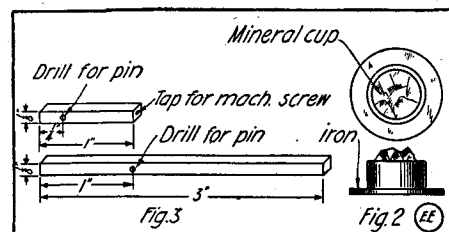
Details of Detector Having Magnetic Cup Retainer.
