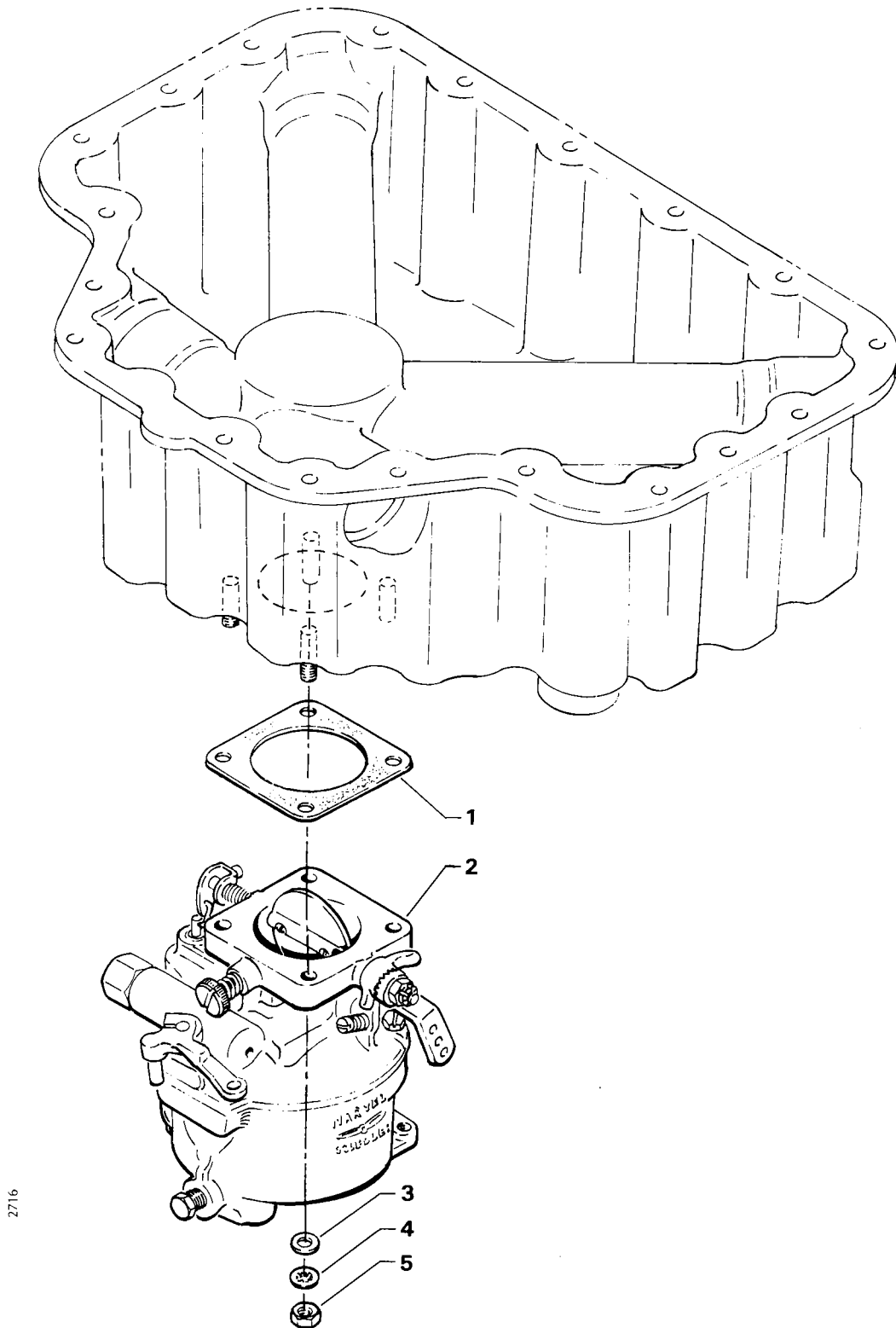
Figure 23. CARBURETOR ASSEMBLY
