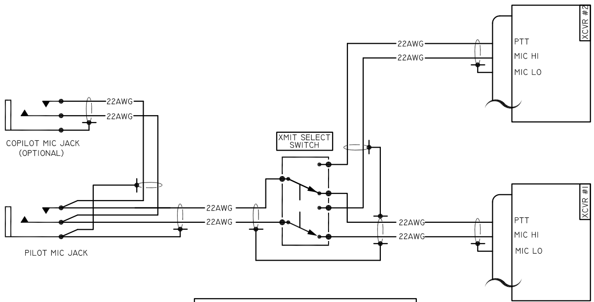
EXEMPLAR TRANSMITTER SELECTOR SWITCH WIRING
