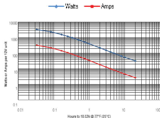
PC1100 performance data at 77°F, per 12V module
