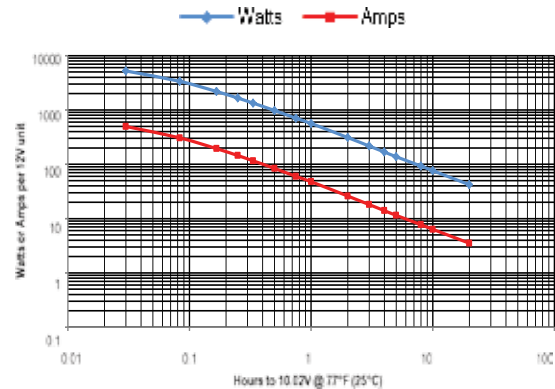
34-PC1500, 34R-PC1500, 34M-PC1500, 34/78-PC1500 and 78-PC1500 performance data at 77°F, per 12V module
