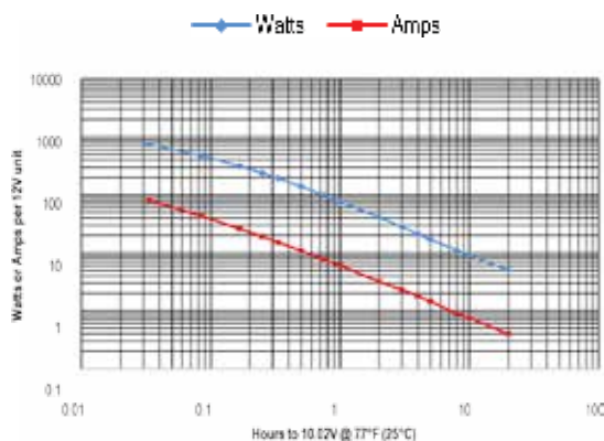
PC310 performance data at 77°F, per 12V module
