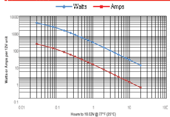
34-790, 34R-790 and 78-790 performance data at 77°F, per 12V module
