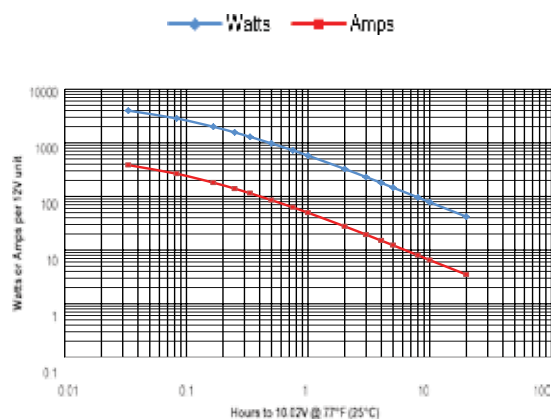
PC1220* performance data at 77°F, per 12V module
