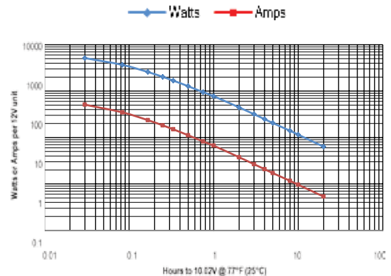
31-800 performance data at 77°F, per 12V module
