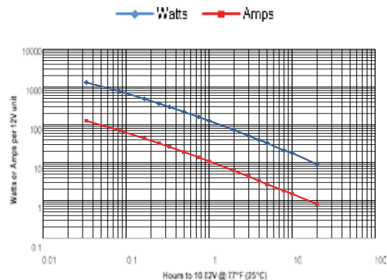
PC370 performance data at 77°F, per 12V module
