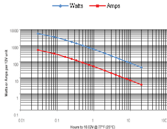
65-PC1750 performance data at 77°F, per 12V module
