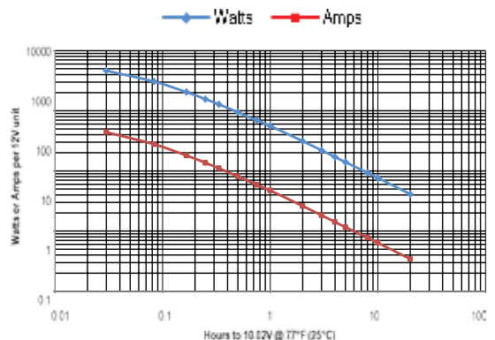
48-720 performance data at 77°F, per 12V module
