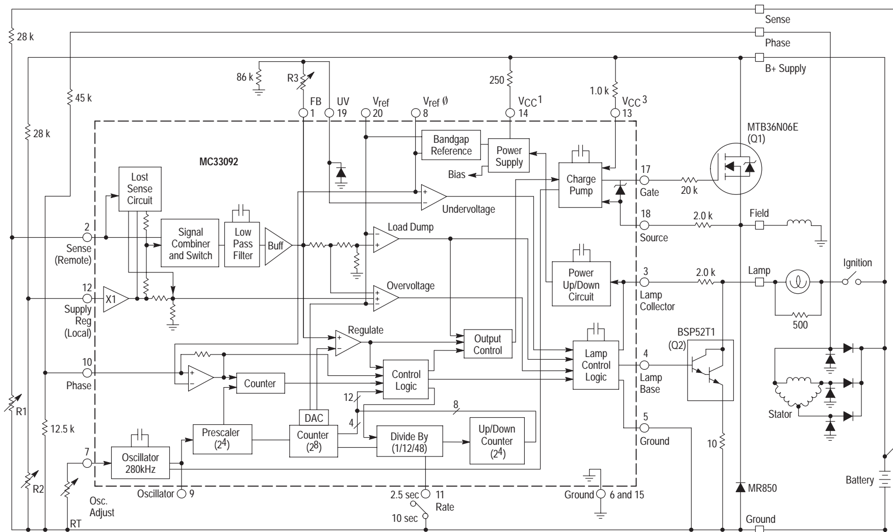
Figure 1. Simplified Application
