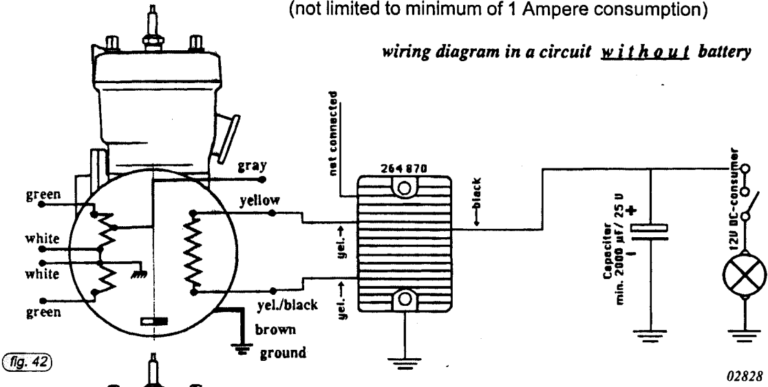
wiring diagram in conjunction with a battery
