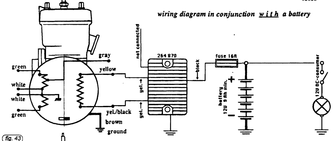
wiring diagram for electric starter
