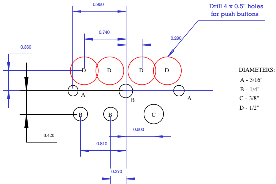
Figure 6-2 Hole Configuration to avoid rectangular cutouts
