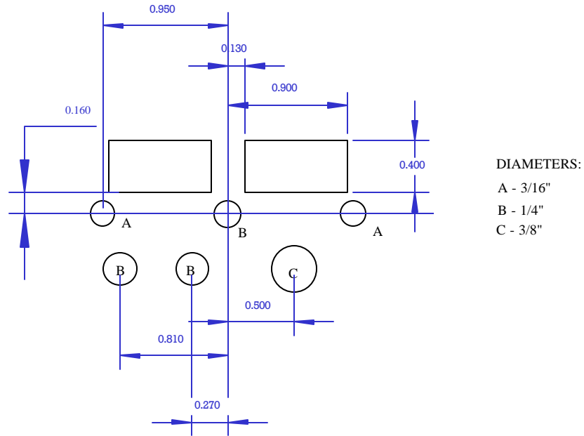
Figure 6-1- Hole Configuration
