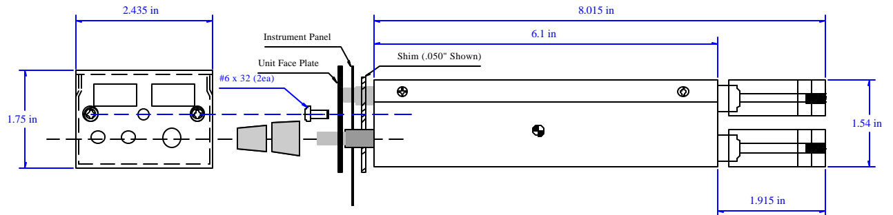
Figure 6-3 Connector Layout
