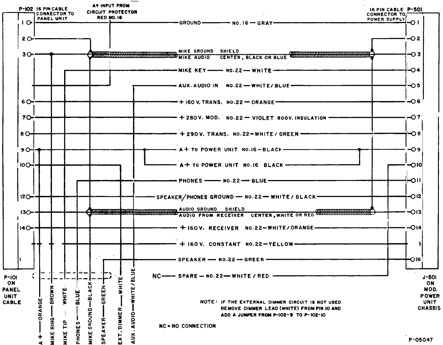
Figure 2-5 MARK 12B TO ACCESSORIES WIRING DIAGRAM
