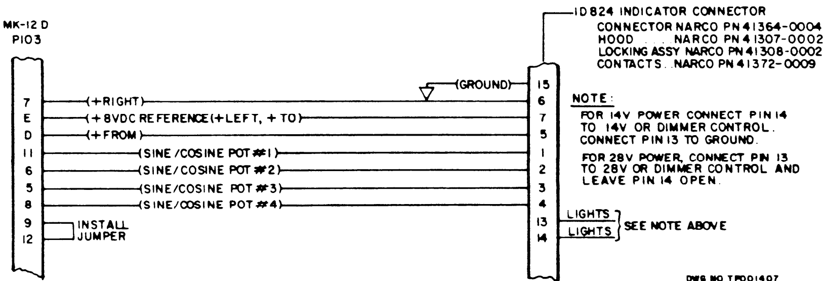
FIGURE 2-11. CABLE WIRING MK-12D WITHOUT GS TO ID 824
