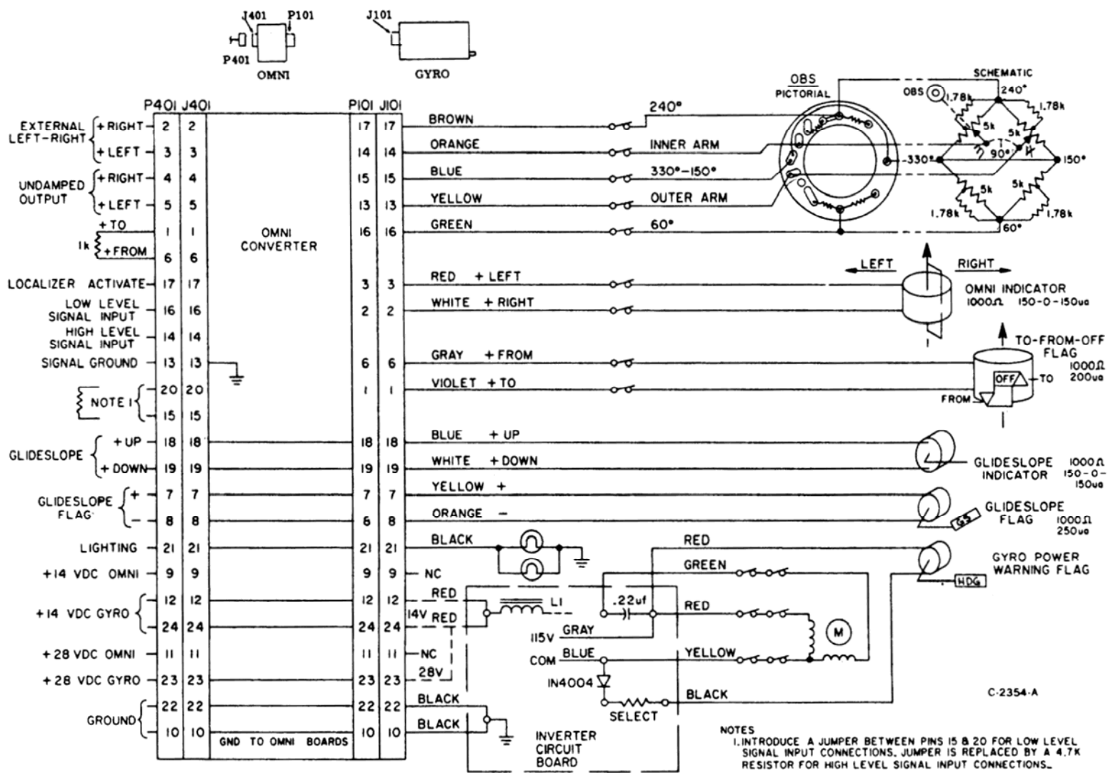
FIGURE 2-4 DGO 10 WIRING AND FUNCTIONAL DIAGRAM
